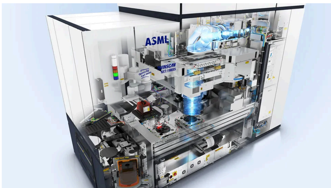
A diagram of an ASML DUV machine. (Image credit: ASML)
